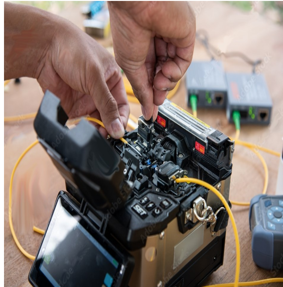
Technician splicing fiber cores
